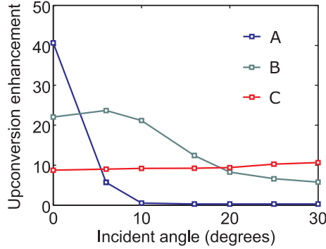
Figure 8.9: 980 nm upconversion enhancement as a function of incident angle for three different annular aperture arrays specified in Fig. 8.8 (1480 nm pump at 16 \text{ W/cm}^2 ). The field enhancement that is caused by a localized resonance (array C) is independent of the angle of incidence.
