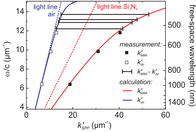
Figure 2.6: Dispersion relations of the two SPP modes that are supported by the system. Closed and open symbols indicate the measured values of k'_{\text{MIM}} and k'_{\text{air}} , respectively. The length of the horizontal bars at high frequencies is equal to the experimentally-determined values of \Delta k' . The solid blue and red lines are the calculated dispersion curves for the air- and MIM-SPP modes, respectively.
