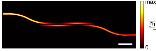
Figure 10.4: Field intensity |E_z|^2 for the directional coupler depicted in Fig. 10.3(a), calculated with the FDTD method in the xy plane in the center of the \text{Si}_3\text{N}_4 slab. The minimum waveguide separation is a = 350 nm, and the free-space wavelength is 1550 nm. SPPs are launched in the nanowire shown in the top left. The intensity in the bottom output nanowire on the right is 100 times larger than that in the top input nanowire. The scale bar is 2 \mu\text{m} .
