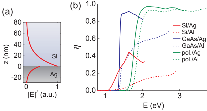
Figure 10.5: (a) Electric field intensity profile of a SPP mode at a Ag/Si interface at a free-space wavelength of 785 nm. (b) Fraction of power absorbed in the active medium as a function of photon energy for SPP modes on different metal/semiconductor interfaces. The metals are Ag (solid curves) and Al (dashed curves). The semiconductors are crystalline Si, GaAs, and a polymer blend (pol.) of PF10TBT:[C60]PCBM [242]. The curves are drawn for energies up to the surface plasmon resonance frequency.
