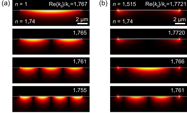
Figure 6.4: Mode profiles of |E| of the four lowest order bound modes guided by a 12\ \mu\text{m} wide and 100\ \text{nm} thick Au waveguide on a sapphire substrate ( n = 1.74 ). The refractive index of the superstrate is changed from n = 1 (a) to n = 1.515 (b).
