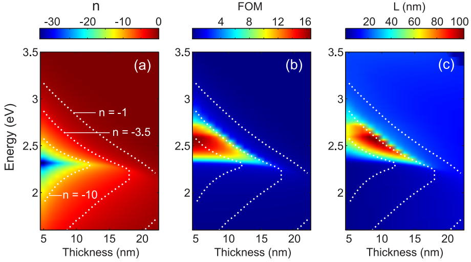
Figure 3.8: Refractive index (a), FOM (b), and propagation length (c) of the negative index mode in a air/GaP/Ag IIM waveguide, for varying GaP thickness and photon energy.
