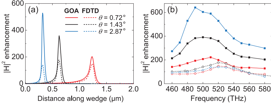
Figure 7.4: Comparison of the |H|^2 intensity enhancements obtained in the GOA (full curves) and in FDTD simulations (dashed curves). (a) Spatial dependence of the magnetic field intensity enhancement along wedges of three different angles, at a frequency of 520 THz. (b) Spectral dependence of the maximum magnetic field intensity enhancement on the wedges, for the same angles as in (a).
