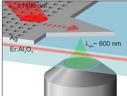
Figure 4.2: Schematic representation of the measurement principle. SPPs are excited at the Ag-sapphire interface by illuminating a hole array with light with a free-space wavelength of 1490 nm, and Er upconversion luminescence at visible frequencies is imaged with a confocal microscope.
