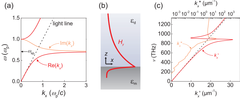
Figure 1.1: (a) Dispersion of SPPs at the interface of a lossless Drude metal with air. (b) Transverse dependence of the H_y field of SPPs on a Ag/air interface. (c) Dispersion of SPPs at the interface of Ag with air. The optical constants are measured on a Ag film [26]. Both the real ( k'_x ) and imaginary ( k''_x ) parts of the wavevector k_x are plotted. The dashed line denotes the light line, \omega = \sqrt{\epsilon_d} c k_x .
