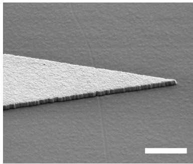
Figure 5.1: SEM micrograph of the end of a fabricated, tapered Au waveguide on an Er-implanted sapphire substrate. The scale bar is 1\text{ }\mu\text{m} .
