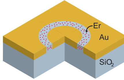
Figure 9.1: Schematic of a single Er-doped SiO 2 annular aperture in a Au film on SiO 2 .
