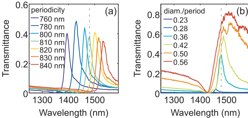
Figure 8.4: (a) Transmission spectra of a hole array in a Au film around the (\pm 1, 0) peak at the \text{Au}/\text{Al}_2\text{O}_3 interface for various array periods. (b) Evolution of the same transmission peak with increasing hole size (indicated as diameter/period). The dashed gray lines depict the wavelength with which Er is excited.
