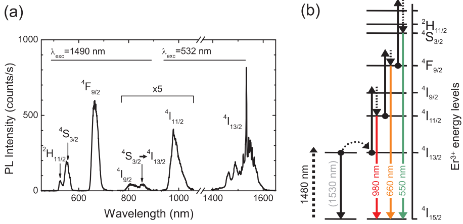
Figure 4.1: (a) Er photoluminescence spectrum showing emission from different Er levels. For \lambda_{\text{em}} < 900 nm, the pump wavelength was 1490 nm, whereas for \lambda_{\text{em}} > 900 nm, 532 nm excitation light was used. The luminescence signal in the region 750–1100 nm is five times enlarged. (b) \text{Er}^{3+} energy level scheme, depicting the cooperative upconversion mechanism that populates higher-order energy levels through energy transfer between two ions excited with 1490 nm light. A multistep upconversion process is shown to reach the levels emitting at 660 and 550 nm.
