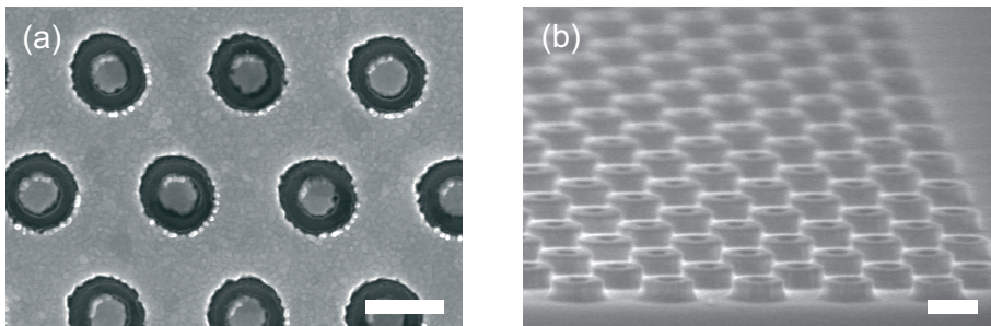
Figure 9.2: (a) SEM image of a fabricated hexagonal array of annular apertures in a Au film. (b) SEM image of Er-doped rings of SiO 2 , not coated with Au. Scale bars are 500 nm.
