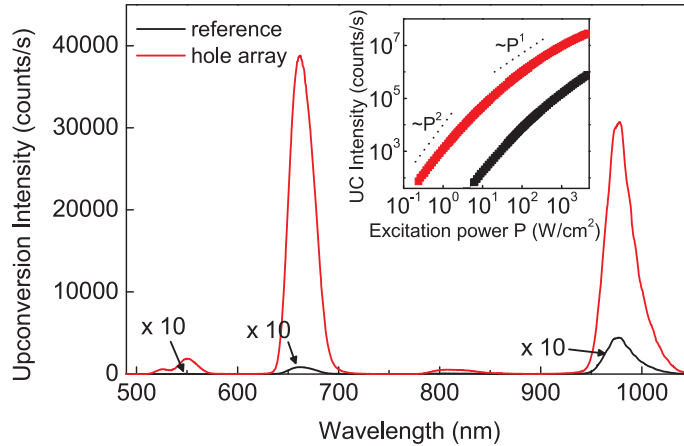
Figure 8.5: Er upconversion spectra obtained from a hole array with a pitch of 810 nm (red) and from a reference in the absence of the Au film (black) under 1480 nm pumping at 200 \text{ W/cm}^2 . Spectral resolution is \sim 20 \text{ nm} . The inset depicts the dependence of the 980 nm emission on 1480 nm pump power, measured on the array (red) and on the reference (black).
